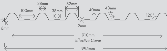
Dimensioned Drawing of Free Span
